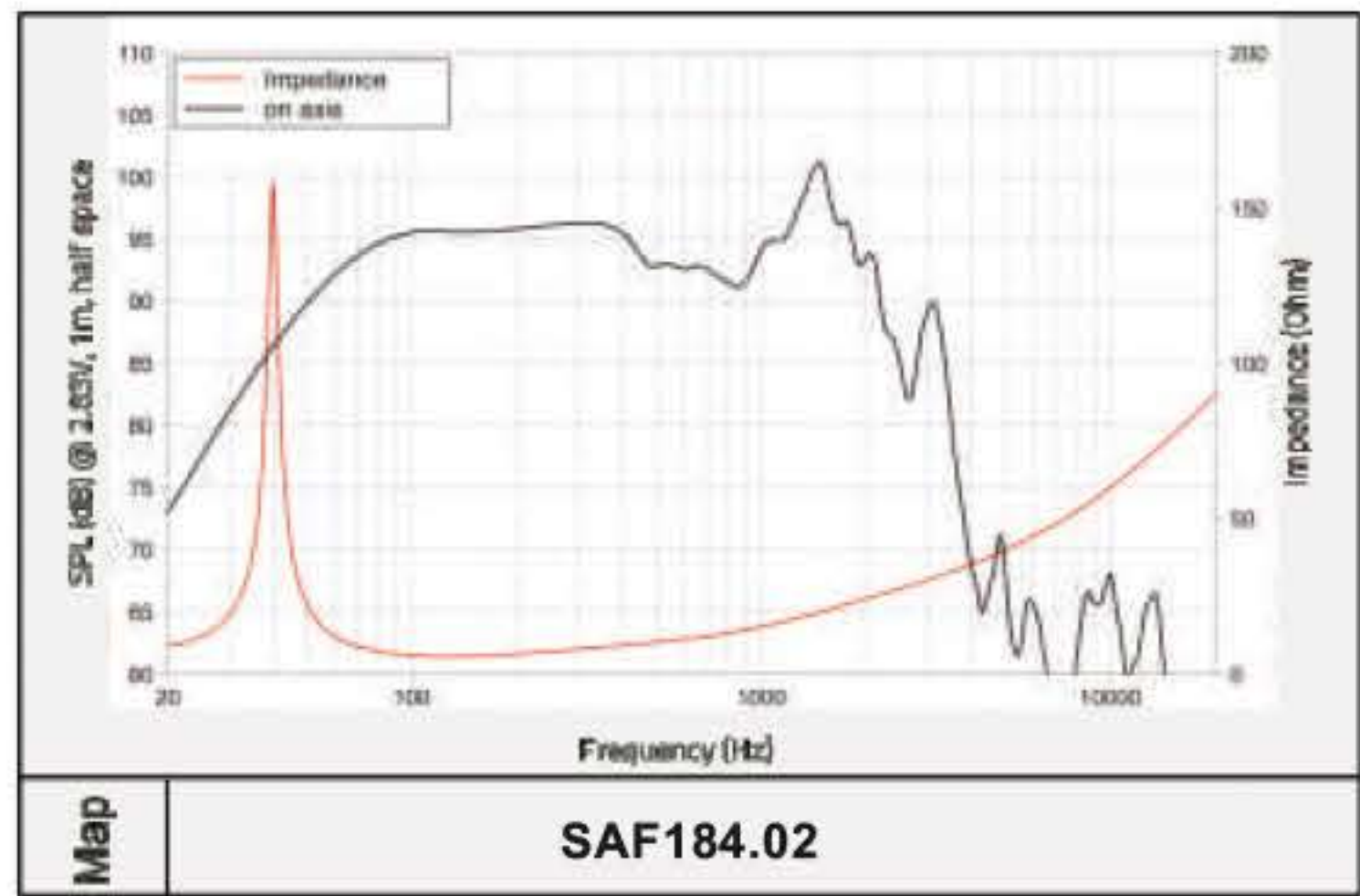
SAF184.02....1200W RMS 4"VC
