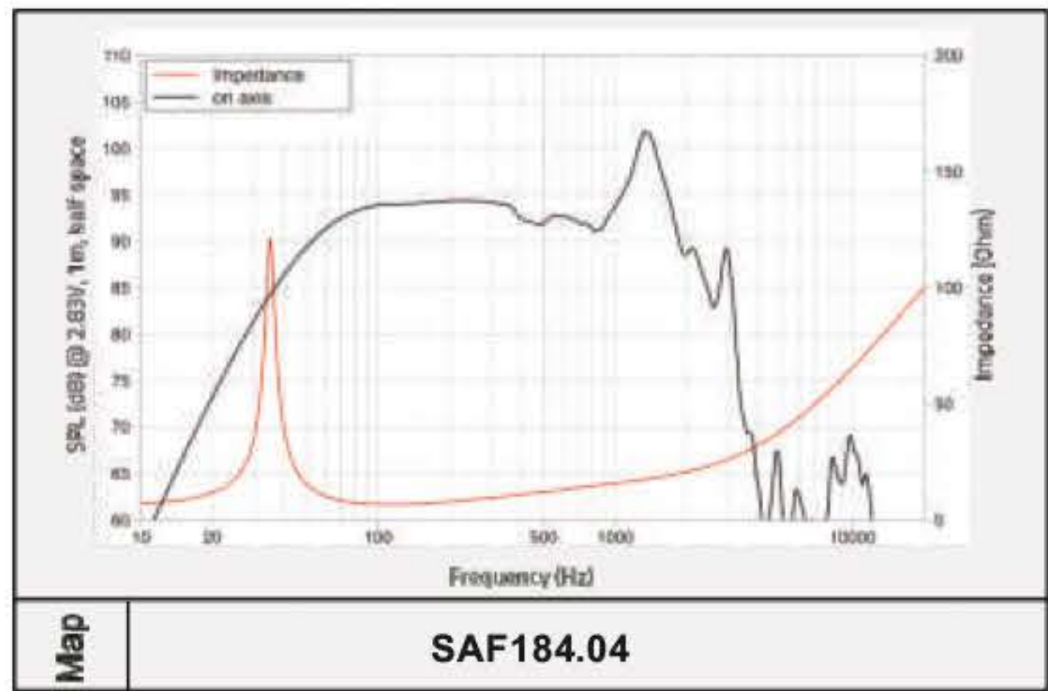
SAF184.04....1500W RMS 4"VC
