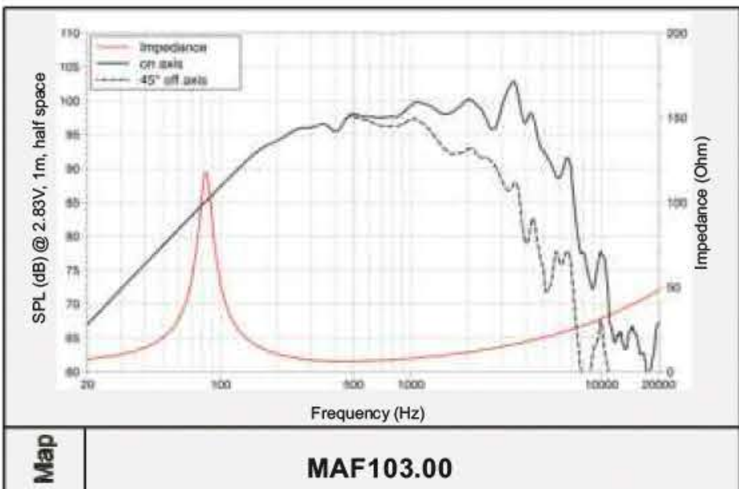
MAF103.00....350W RMS 3"VC
